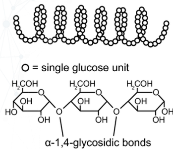
amylose
