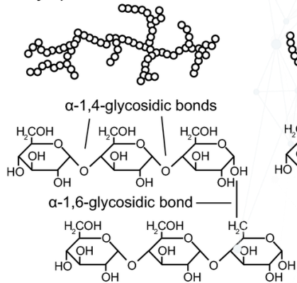
amylopectin
